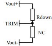
Voltage Down: Add resistor R_{down} between Trim and output positive R_{down} = 24 * (28 - 2.5 - \Delta U) / \Delta U - 5.1 (K \Omega )
