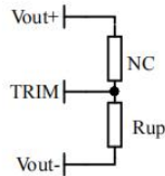
Voltage up regulation: add resistor R_{up} between Trim and output negative R_{up} = 60 / \Delta U - 5.1 (K \Omega )
